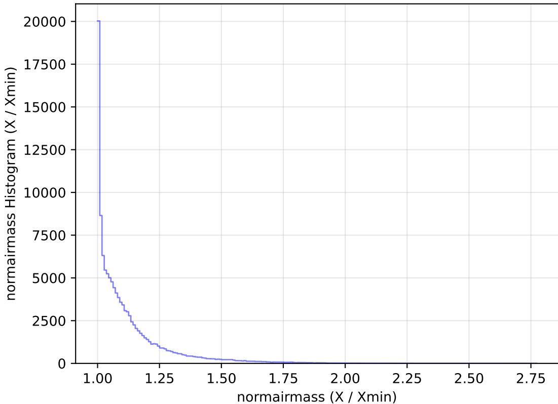
too_elab_r64_d2_gz_v3.4_10yrs All sky u band: normairmass Histogram
