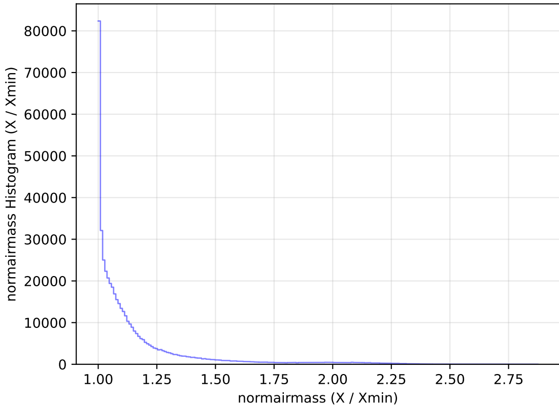
too_elab_r64_d2_gz_v3.4_10yrs All sky r band: normairmass Histogram
