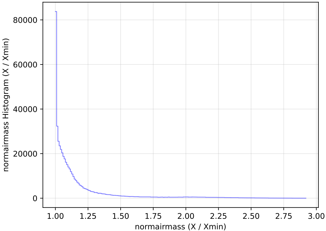
too_elab_r64_d2_gz_v3.4_10yrs All sky i band: normairmass Histogram
