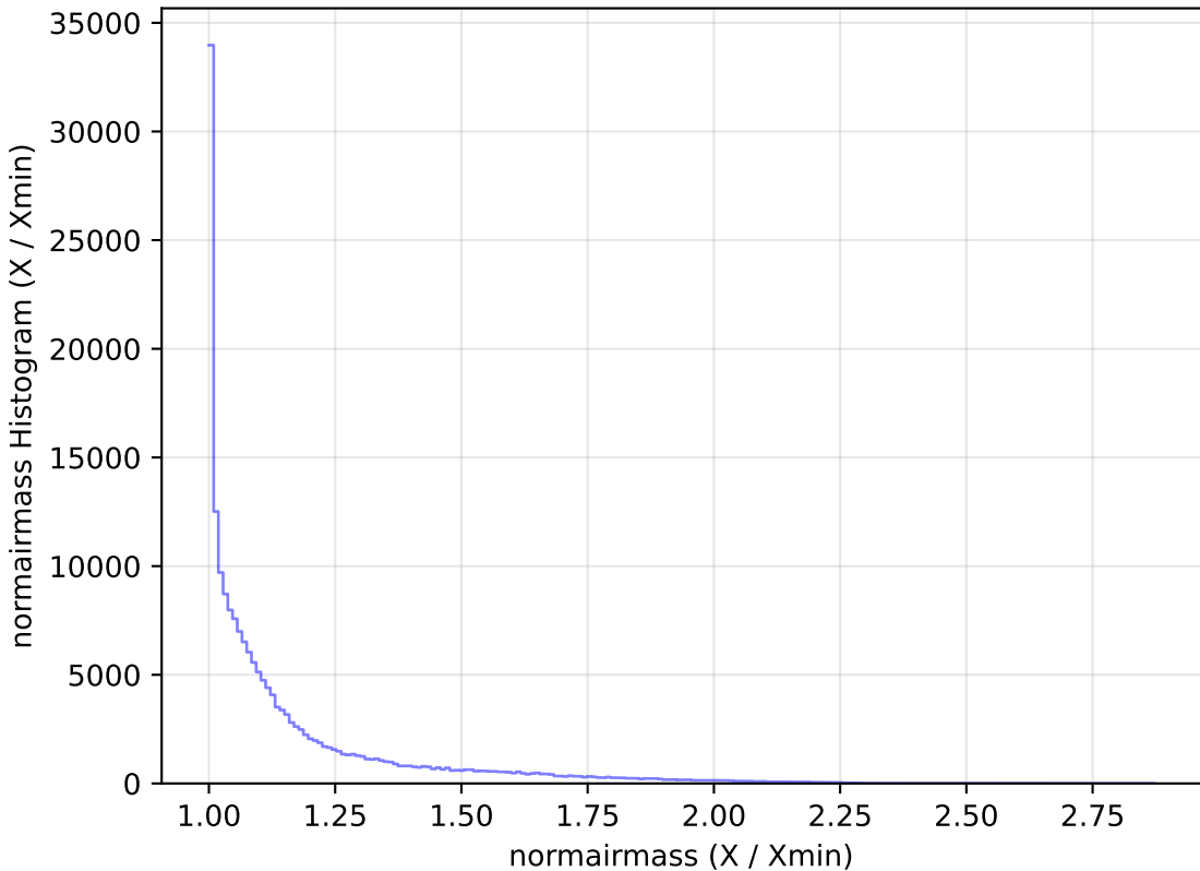
too_elab_r64_d2_gz_v3.4_10yrs All sky g band: normairmass Histogram
