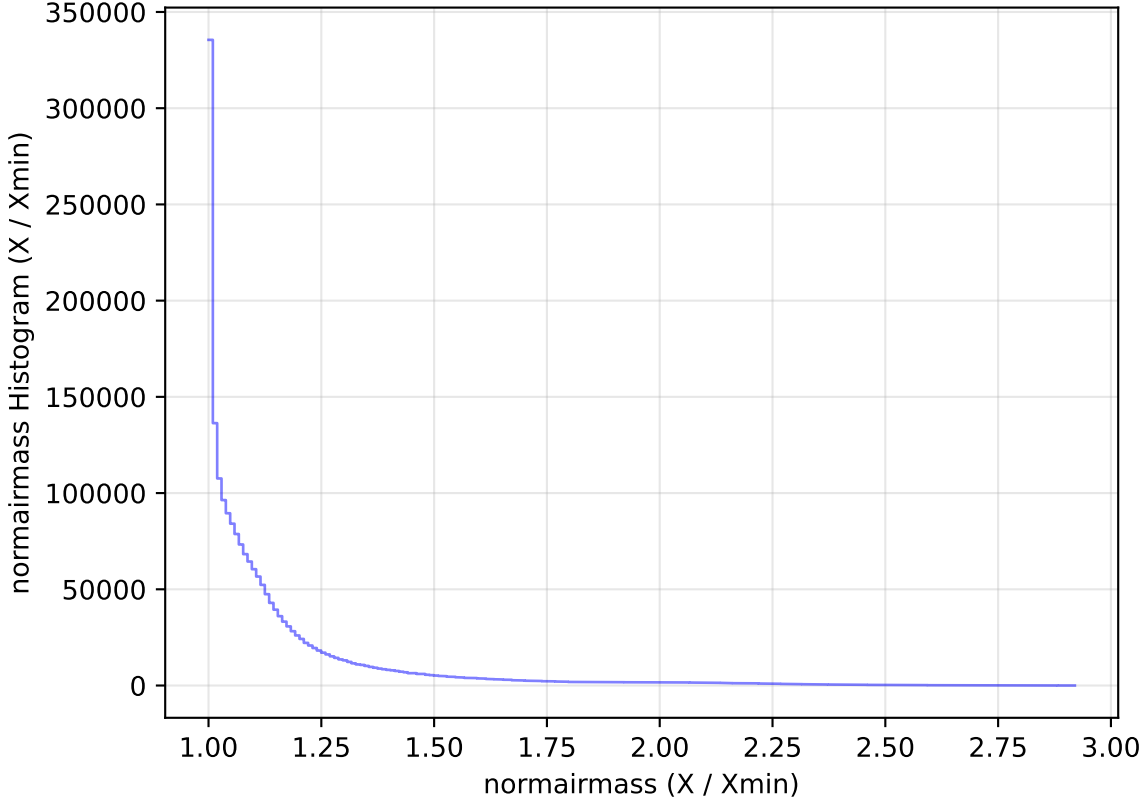
too_elab_r64_d2_gz_v3.4_10yrs All sky all bands: normairmass Histogram
