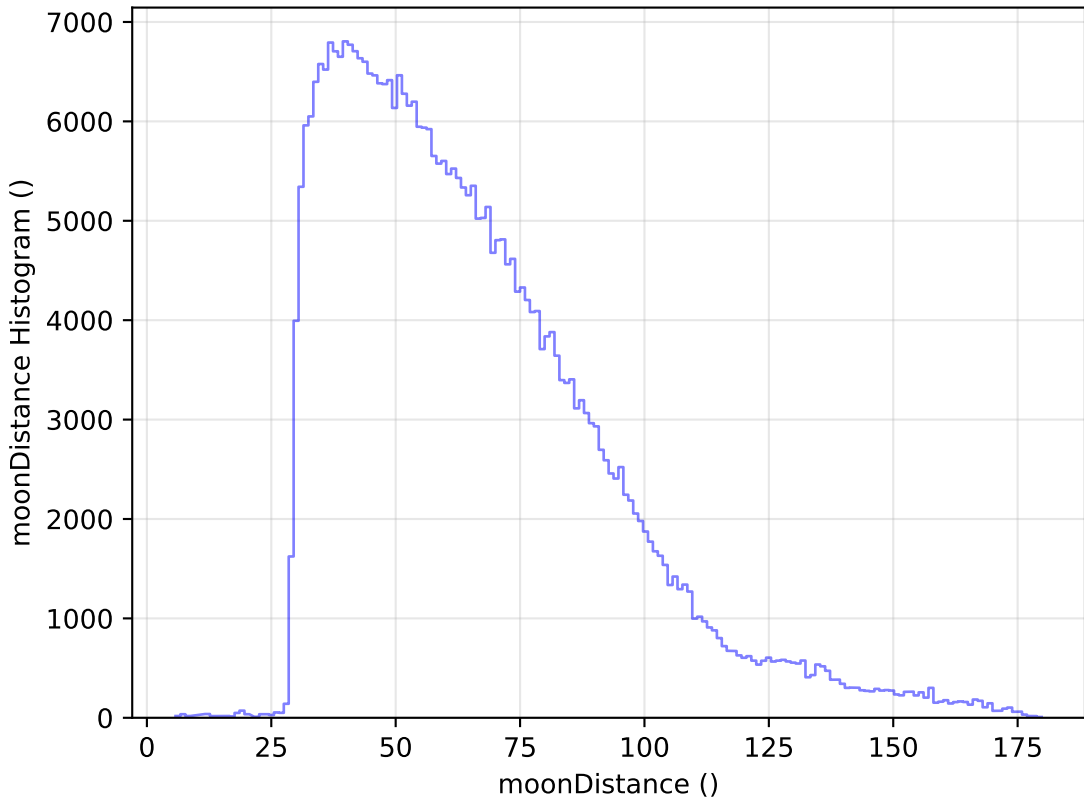
too_elab_r64_d2_gz_v3.4_10yrs WFD y band: moonDistance Histogram
