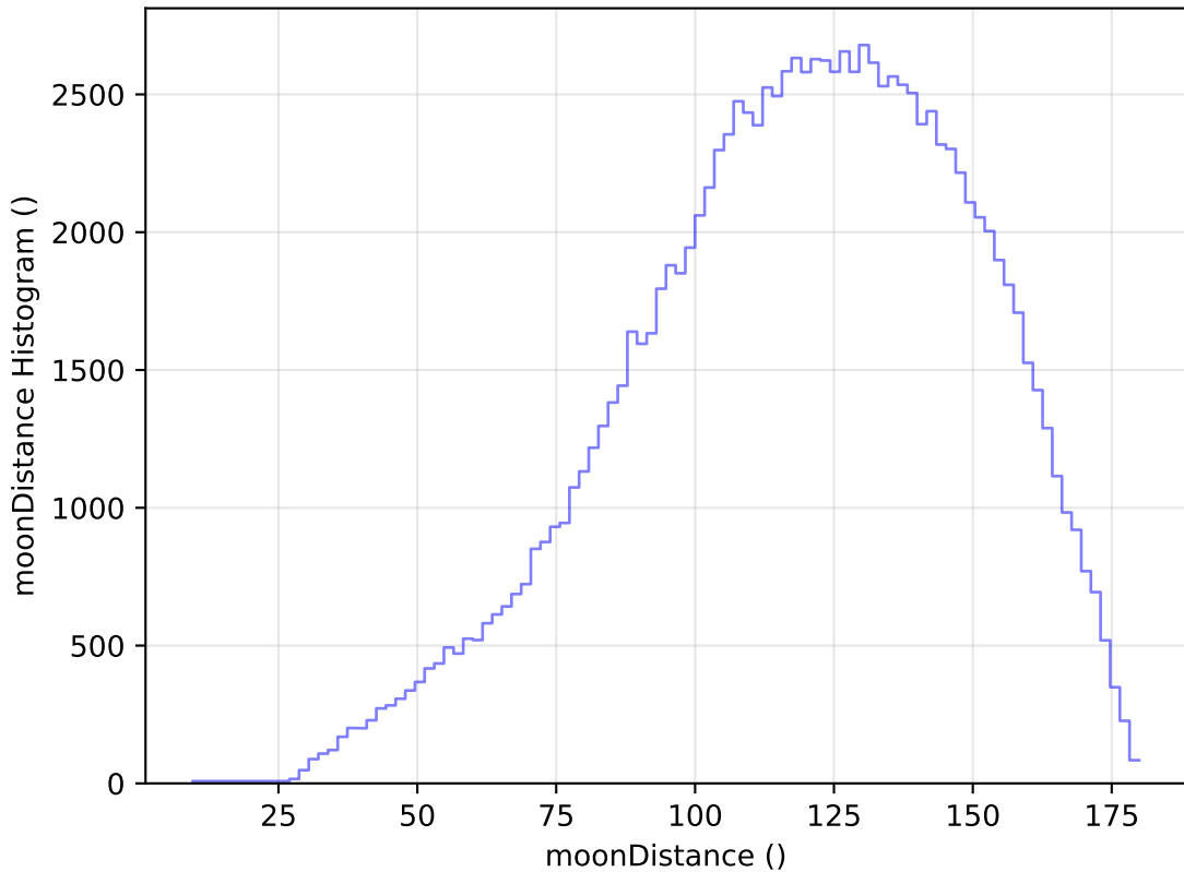
too_elab_r64_d2_gz_v3.4_10yrs WFD u band: moonDistance Histogram
