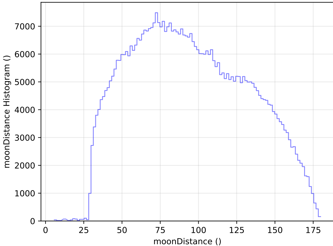
too_elab_r64_d2_gz_v3.4_10yrs WFD i band: moonDistance Histogram
