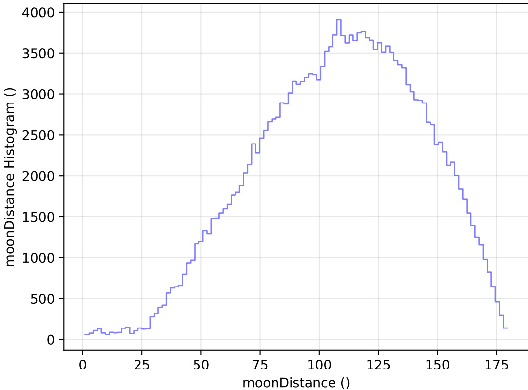
too_elab_r64_d2_gz_v3.4_10yrs WFD g band: moonDistance Histogram
