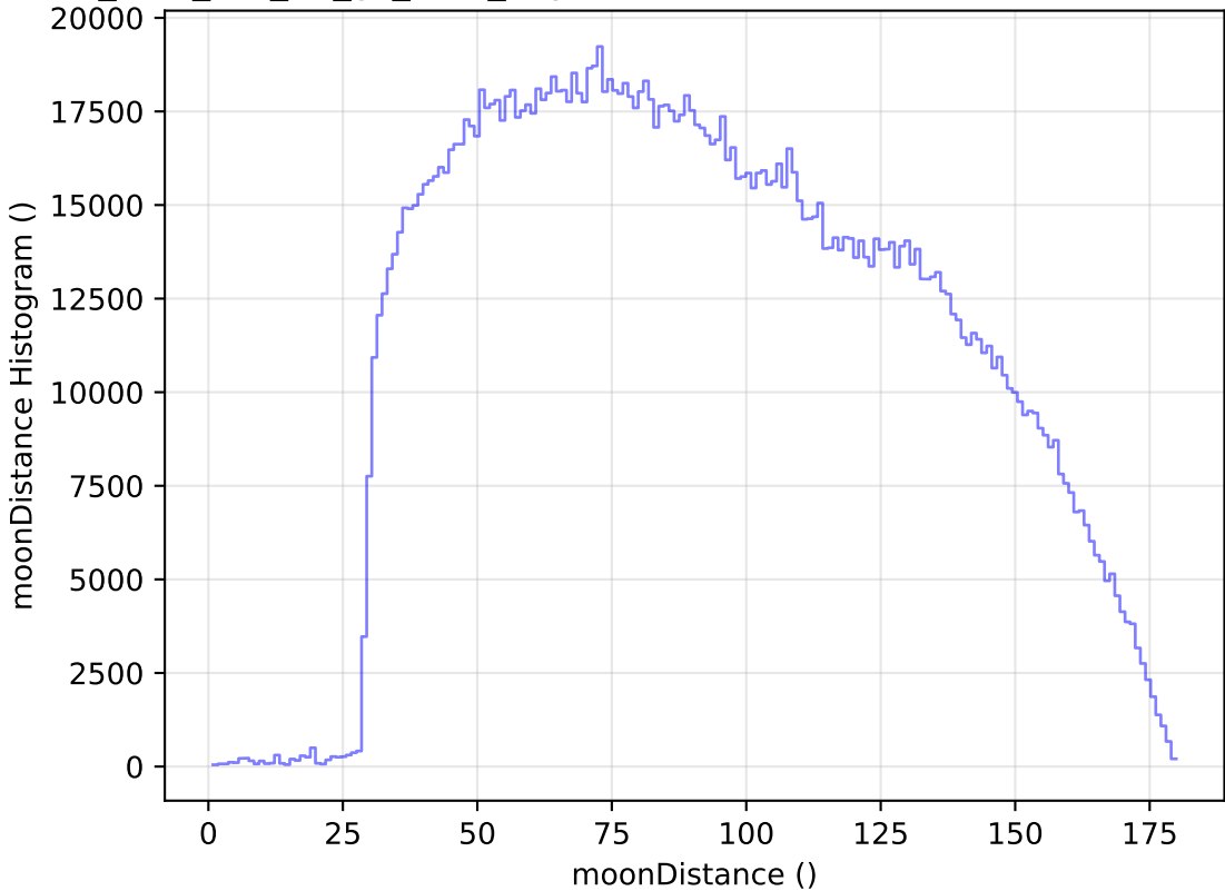
too_elab_r64_d2_gz_v3.4_10yrs WFD all bands: moonDistance Histogram
