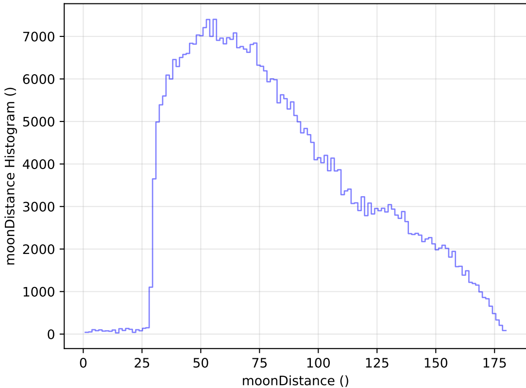
too_elab_r64_d2_gz_v3.4_10yrs All sky z band: moonDistance Histogram
