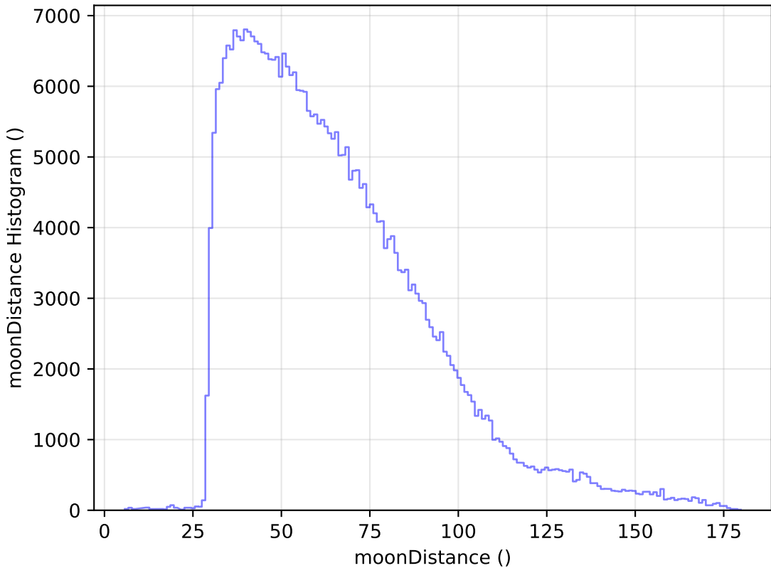
too_elab_r64_d2_gz_v3.4_10yrs All sky y band: moonDistance Histogram
