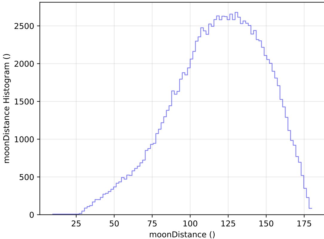
too_elab_r64_d2_gz_v3.4_10yrs All sky u band: moonDistance Histogram
