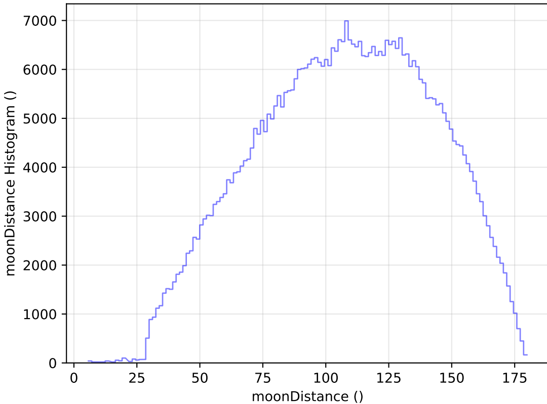
too_elab_r64_d2_gz_v3.4_10yrs All sky r band: moonDistance Histogram
