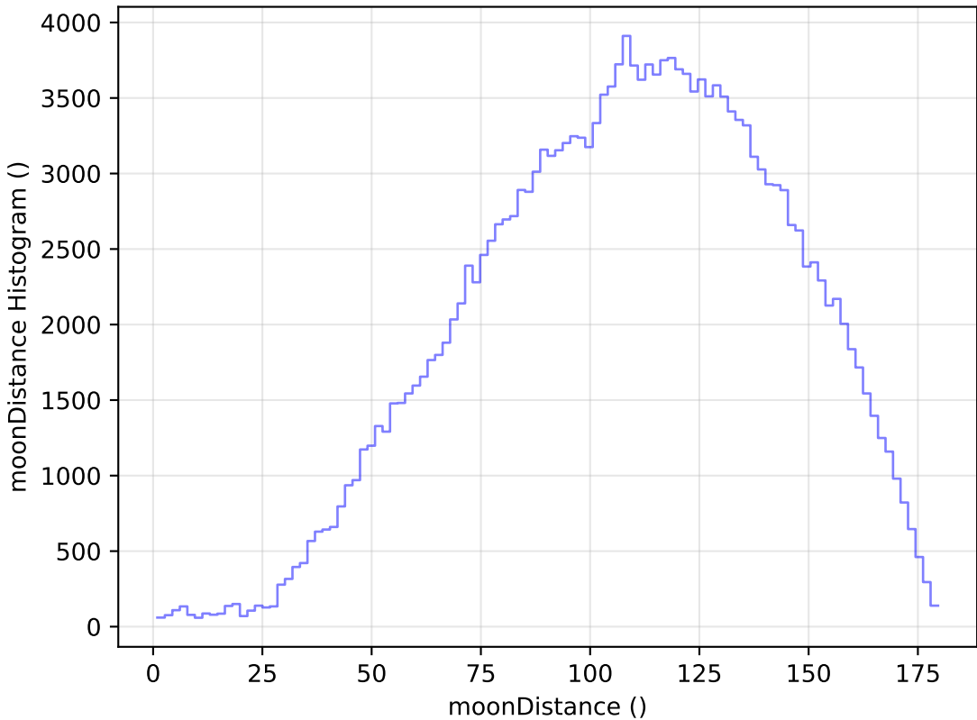
too_elab_r64_d2_gz_v3.4_10yrs All sky g band: moonDistance Histogram
