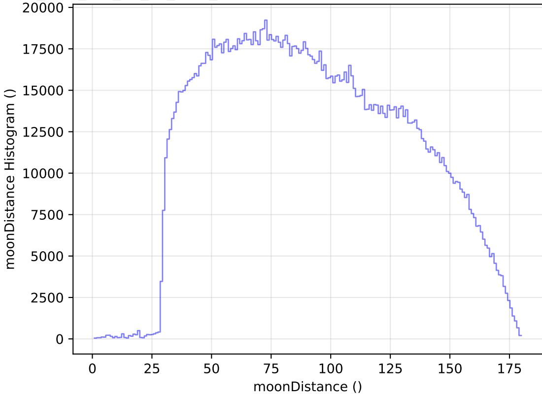
too_elab_r64_d2_gz_v3.4_10yrs All sky all bands: moonDistance Histogram
