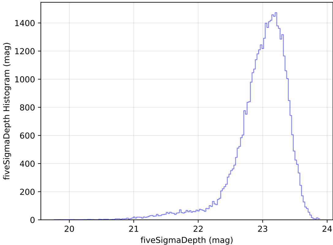
too_elab_r64_d2_gz_v3.4_10yrs Yr 1 z band: fiveSigmaDepth Histogram
