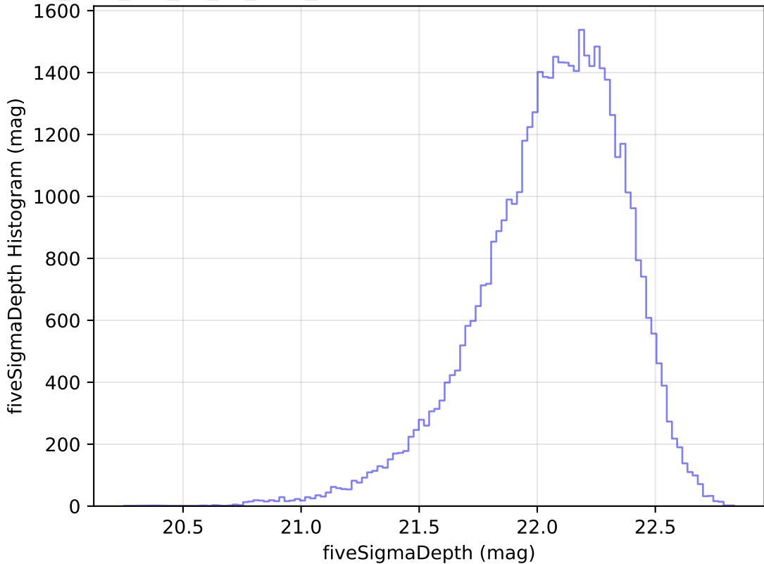
too_elab_r64_d2_gz_v3.4_10yrs Yr 1 y band: fiveSigmaDepth Histogram
