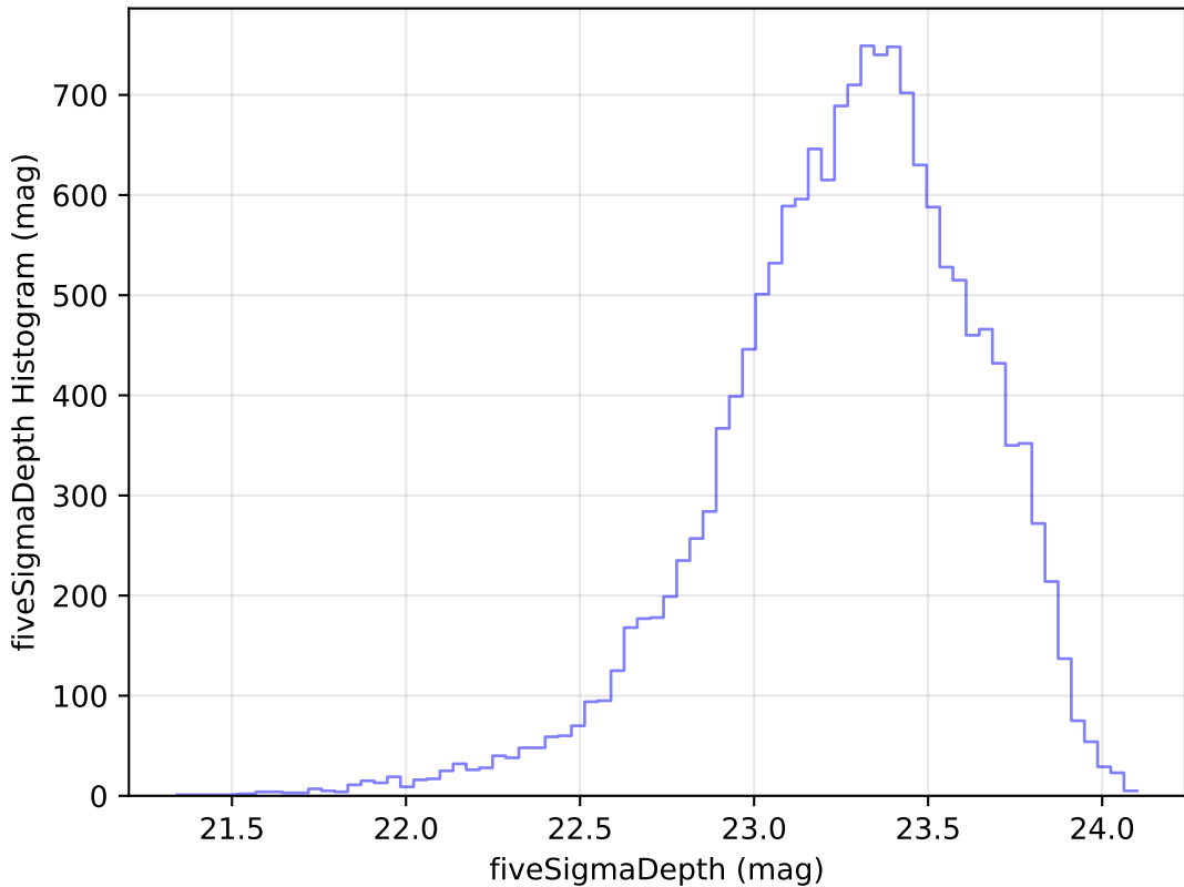
too_elab_r64_d2_gz_v3.4_10yrs Yr 1 u band: fiveSigmaDepth Histogram
