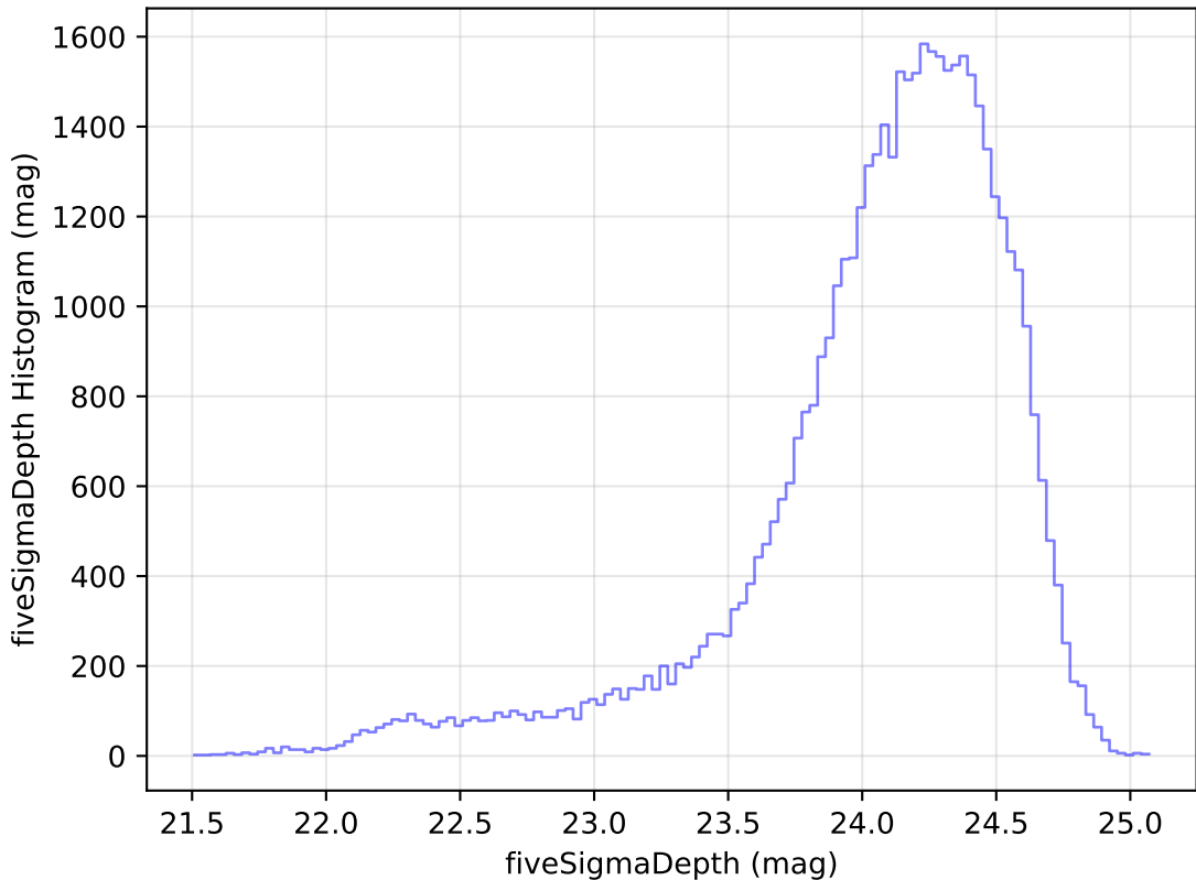
too_elab_r64_d2_gz_v3.4_10yrs Yr 1 r band: fiveSigmaDepth Histogram
