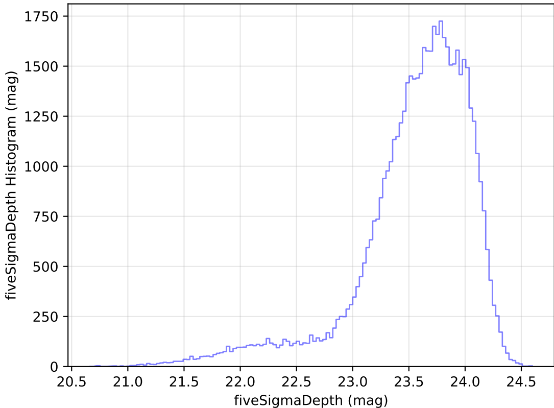
too_elab_r64_d2_gz_v3.4_10yrs Yr 1 i band: fiveSigmaDepth Histogram
