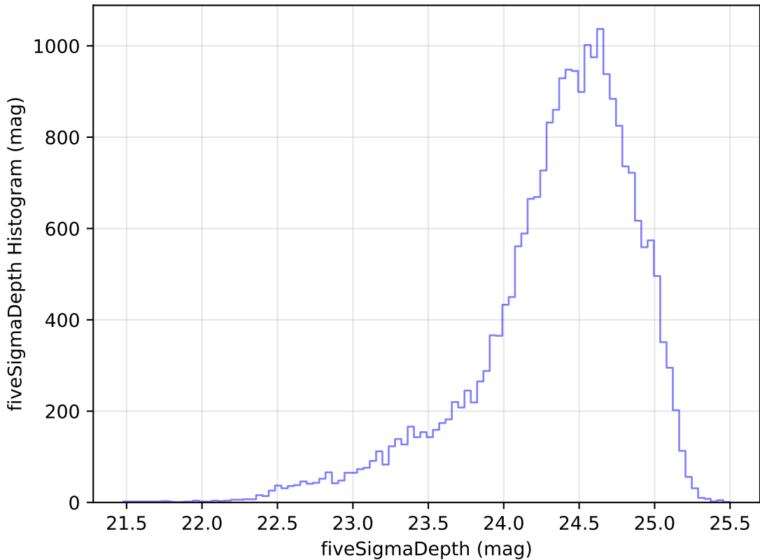
too_elab_r64_d2_gz_v3.4_10yrs Yr 1 g band: fiveSigmaDepth Histogram
