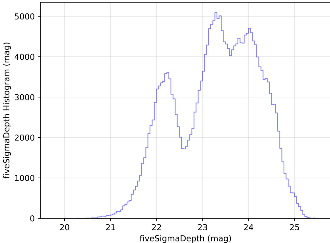
too_elab_r64_d2_gz_v3.4_10yrs Yr 1 all bands: fiveSigmaDepth Histogram
