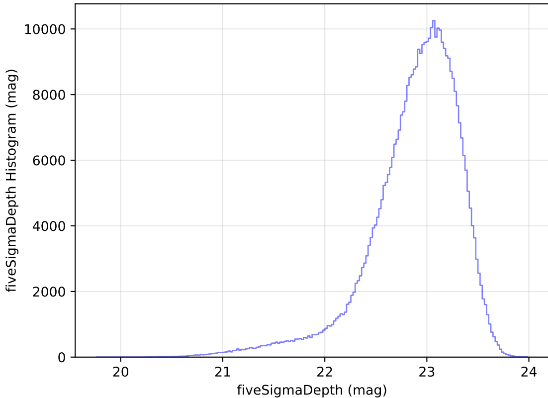
too_elab_r64_d2_gz_v3.4_10yrs WFD z band: fiveSigmaDepth Histogram
