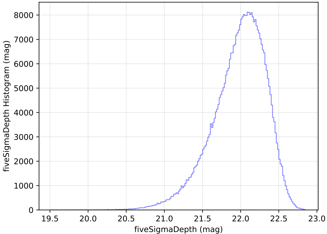
too_elab_r64_d2_gz_v3.4_10yrs WFD y band: fiveSigmaDepth Histogram
