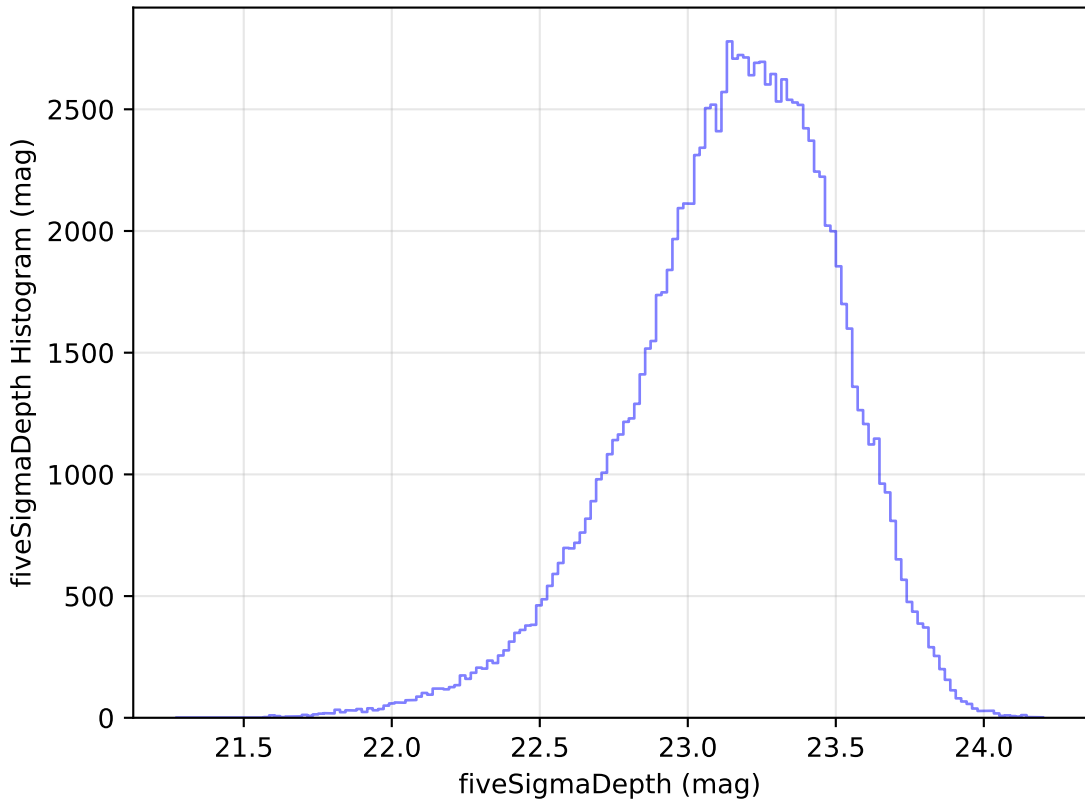
too_elab_r64_d2_gz_v3.4_10yrs WFD u band: fiveSigmaDepth Histogram
