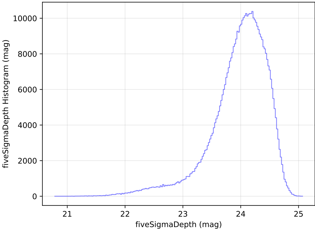
too_elab_r64_d2_gz_v3.4_10yrs WFD r band: fiveSigmaDepth Histogram
