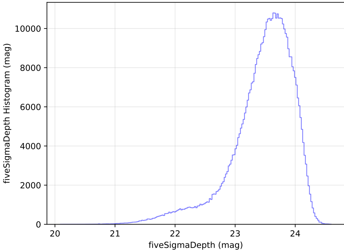
too_elab_r64_d2_gz_v3.4_10yrs WFD i band: fiveSigmaDepth Histogram
