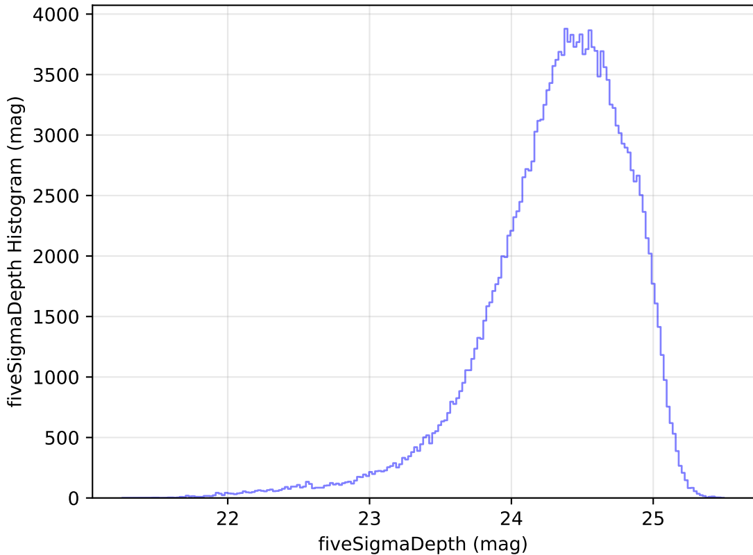
too_elab_r64_d2_gz_v3.4_10yrs WFD g band: fiveSigmaDepth Histogram
