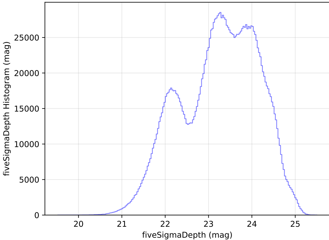
too_elab_r64_d2_gz_v3.4_10yrs WFD all bands: fiveSigmaDepth Histogram
