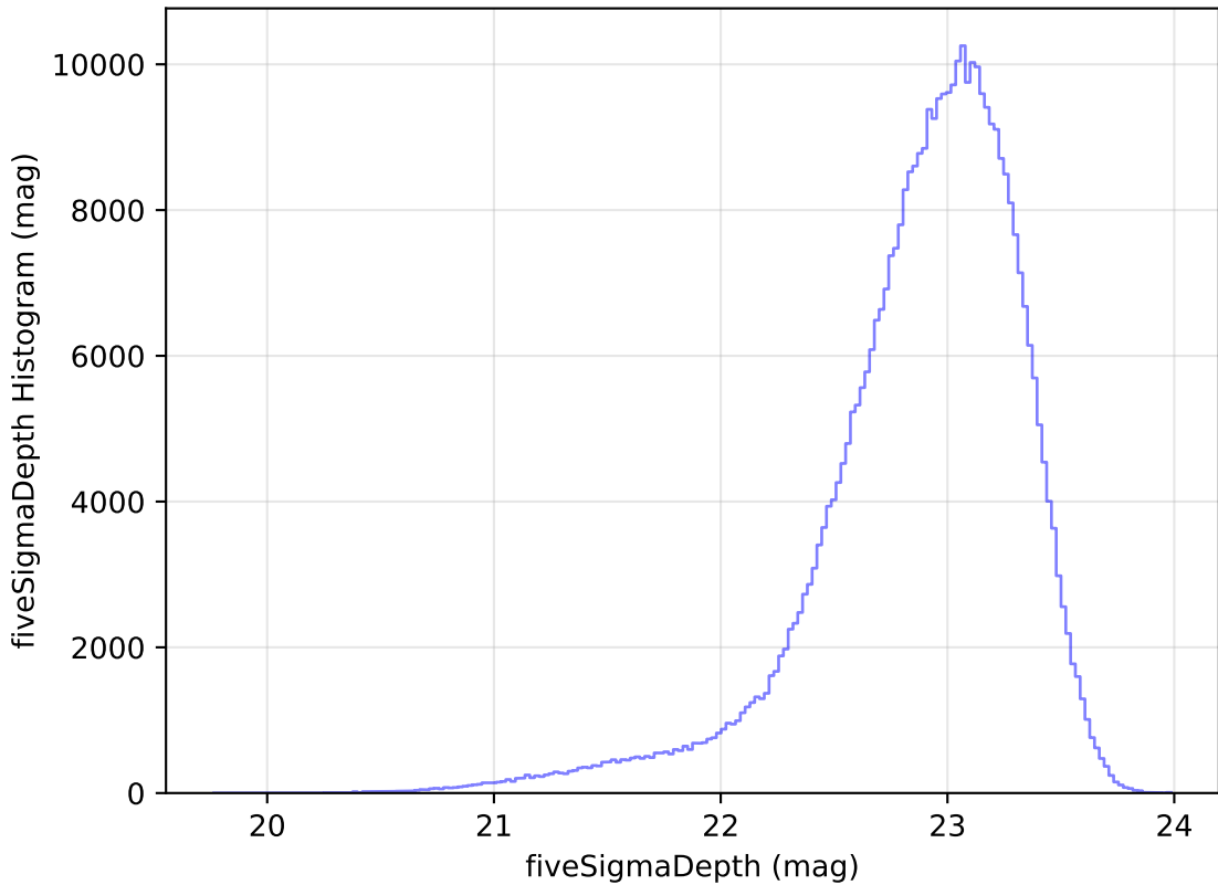
too_elab_r64_d2_gz_v3.4_10yrs All sky z band: fiveSigmaDepth Histogram
