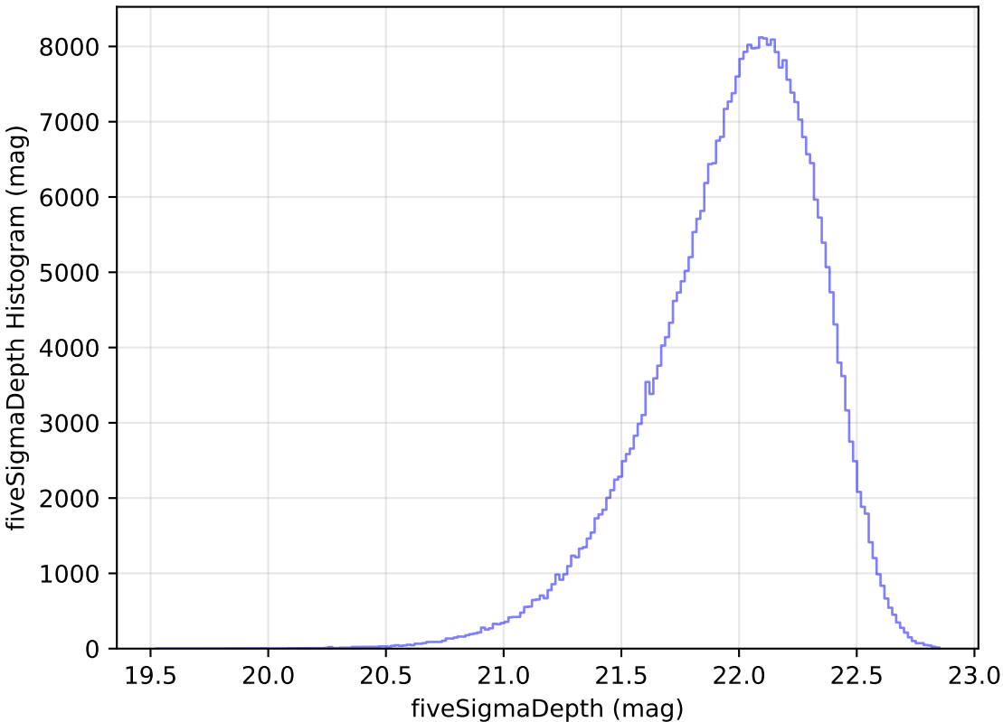
too_elab_r64_d2_gz_v3.4_10yrs All sky y band: fiveSigmaDepth Histogram
