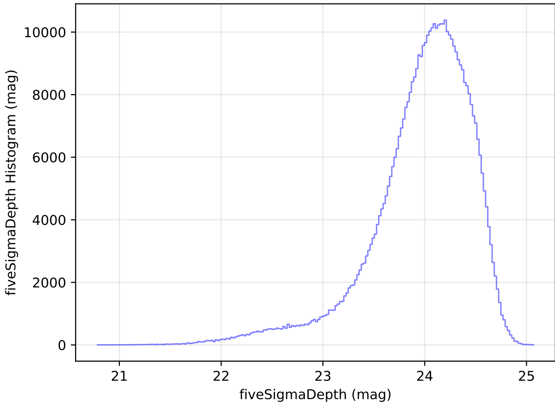
too_elab_r64_d2_gz_v3.4_10yrs All sky r band: fiveSigmaDepth Histogram
