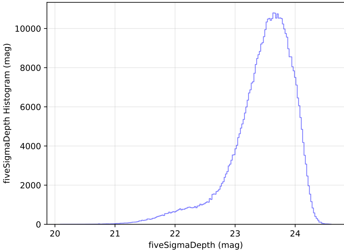
too_elab_r64_d2_gz_v3.4_10yrs All sky i band: fiveSigmaDepth Histogram
