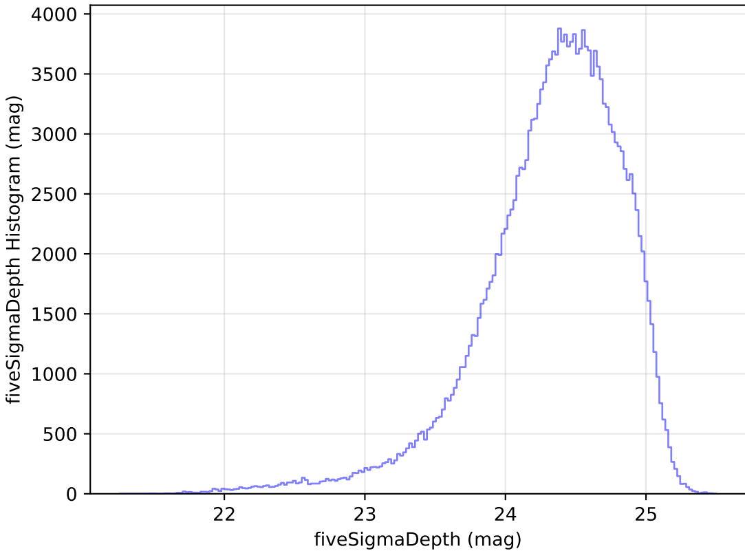
too_elab_r64_d2_gz_v3.4_10yrs All sky g band: fiveSigmaDepth Histogram
