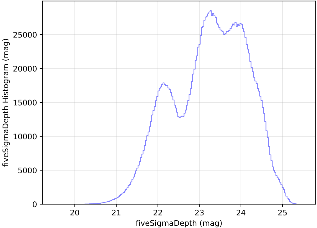
too_elab_r64_d2_gz_v3.4_10yrs All sky all bands: fiveSigmaDepth Histogram
