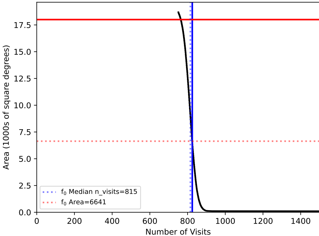
too_elab_r64_d2_gz_v3.4_10yrs WFD: f0
