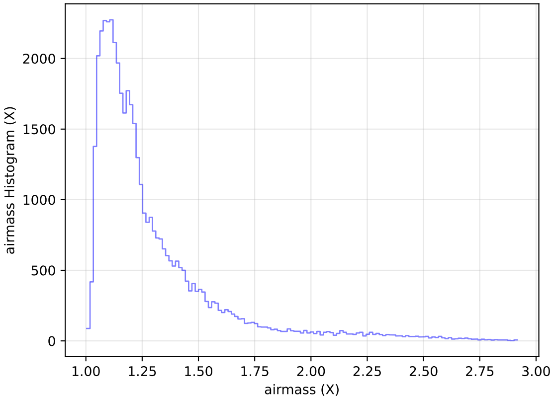
too_elab_r64_d2_gz_v3.4_10yrs Yr 1 z band: airmass Histogram
