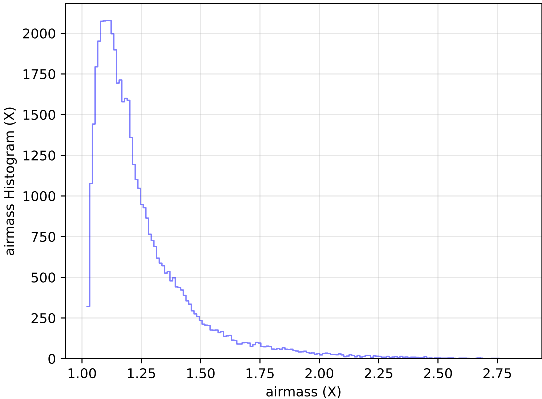
too_elab_r64_d2_gz_v3.4_10yrs Yr 1 y band: airmass Histogram
