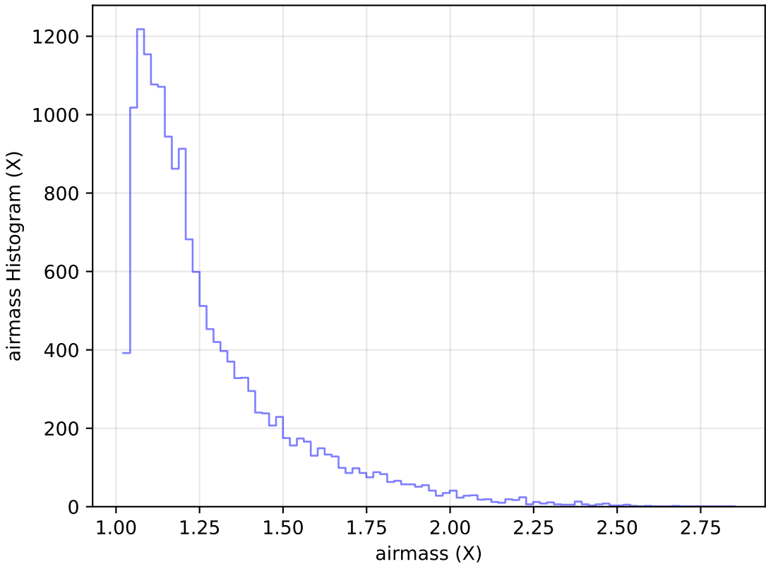
too_elab_r64_d2_gz_v3.4_10yrs Yr 1 u band: airmass Histogram
