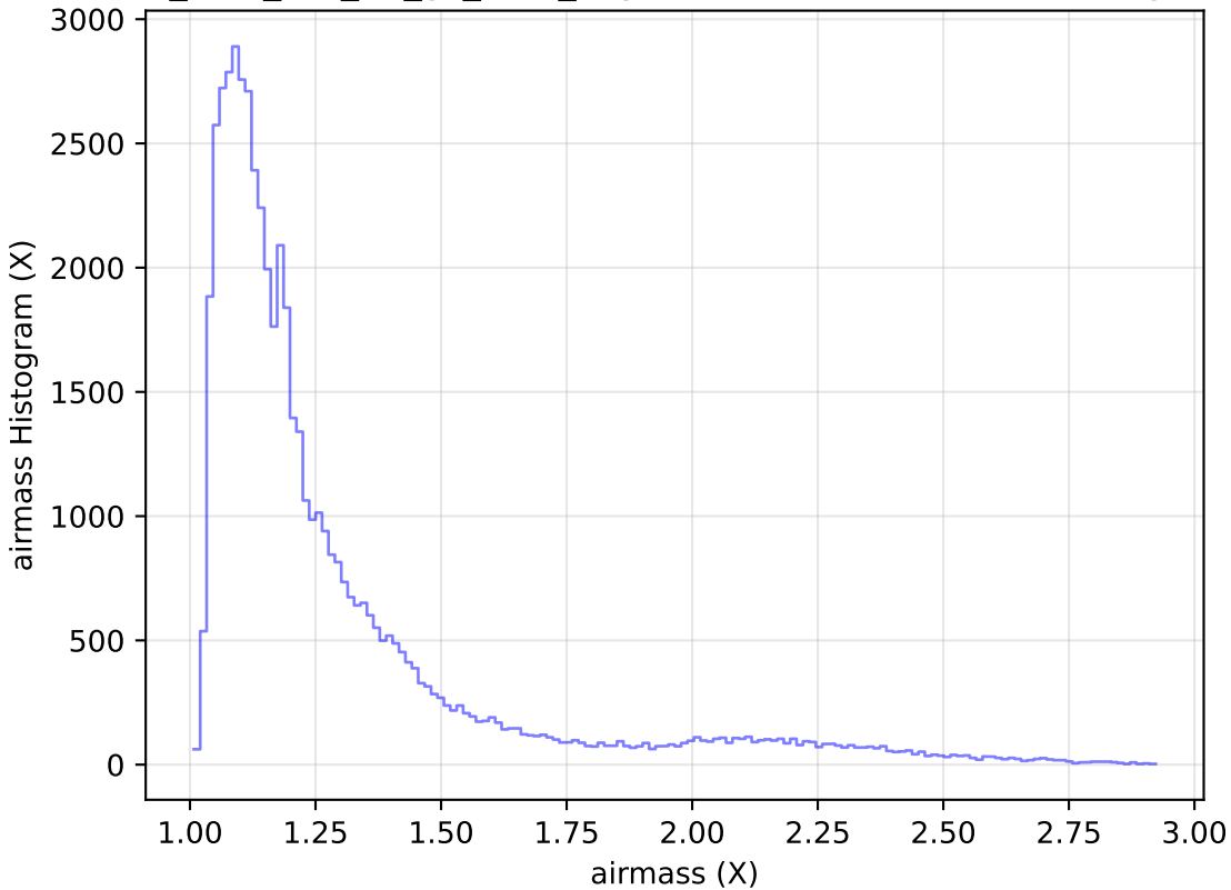
too_elab_r64_d2_gz_v3.4_10yrs Yr 1 i band: airmass Histogram
