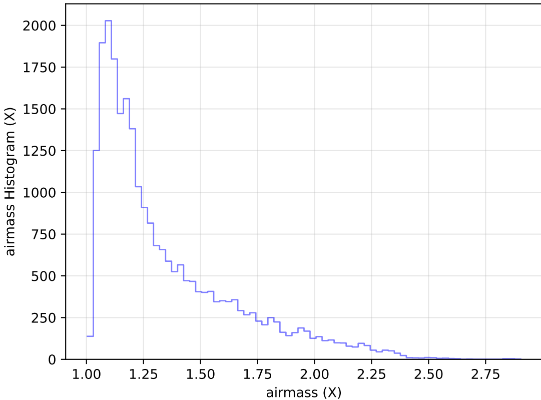
too_elab_r64_d2_gz_v3.4_10yrs Yr 1 g band: airmass Histogram
