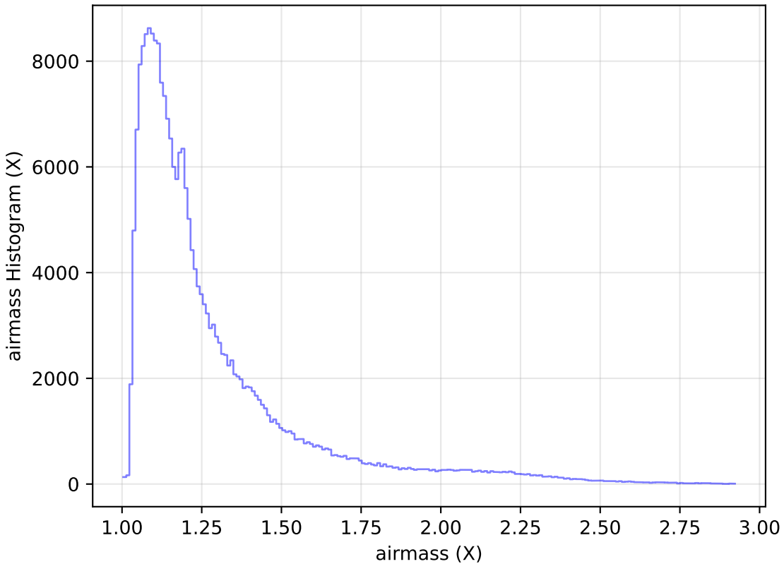
too_elab_r64_d2_gz_v3.4_10yrs Yr 1 all bands: airmass Histogram
