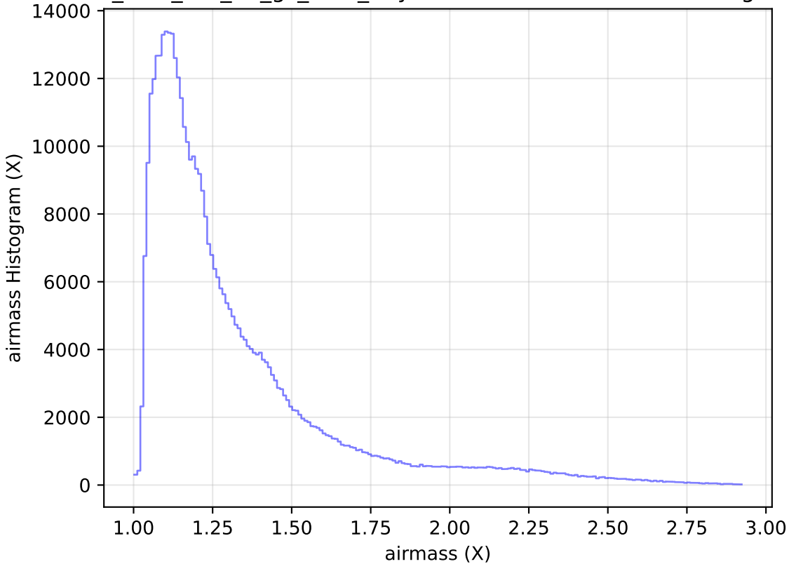
too_elab_r64_d2_gz_v3.4_10yrs WFD z band: airmass Histogram
