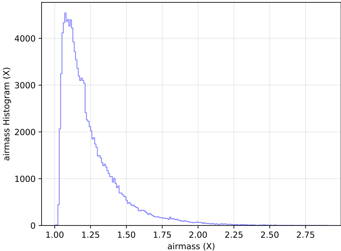
too_elab_r64_d2_gz_v3.4_10yrs WFD u band: airmass Histogram
