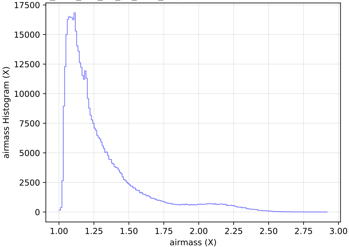
too_elab_r64_d2_gz_v3.4_10yrs WFD r band: airmass Histogram
