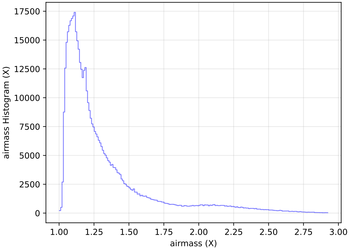
too_elab_r64_d2_gz_v3.4_10yrs WFD i band: airmass Histogram
