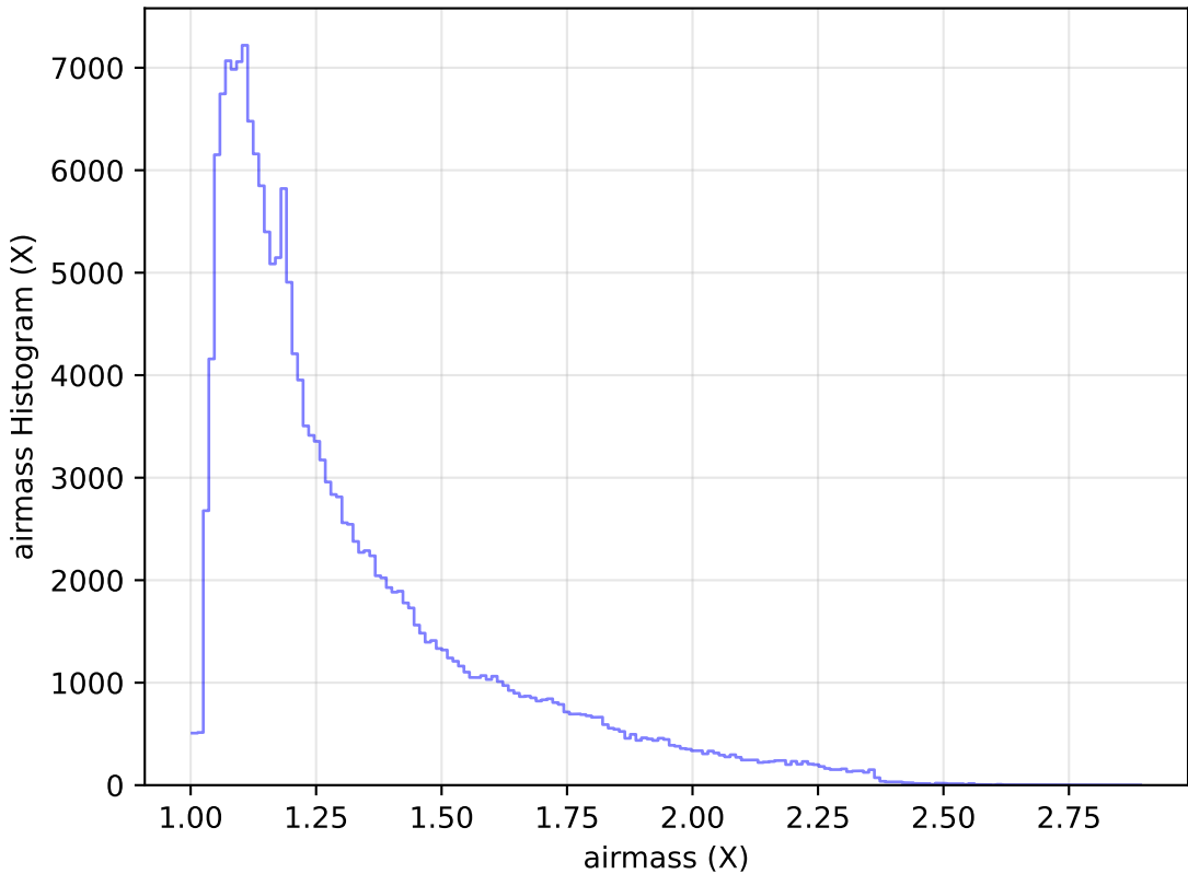
too_elab_r64_d2_gz_v3.4_10yrs WFD g band: airmass Histogram
