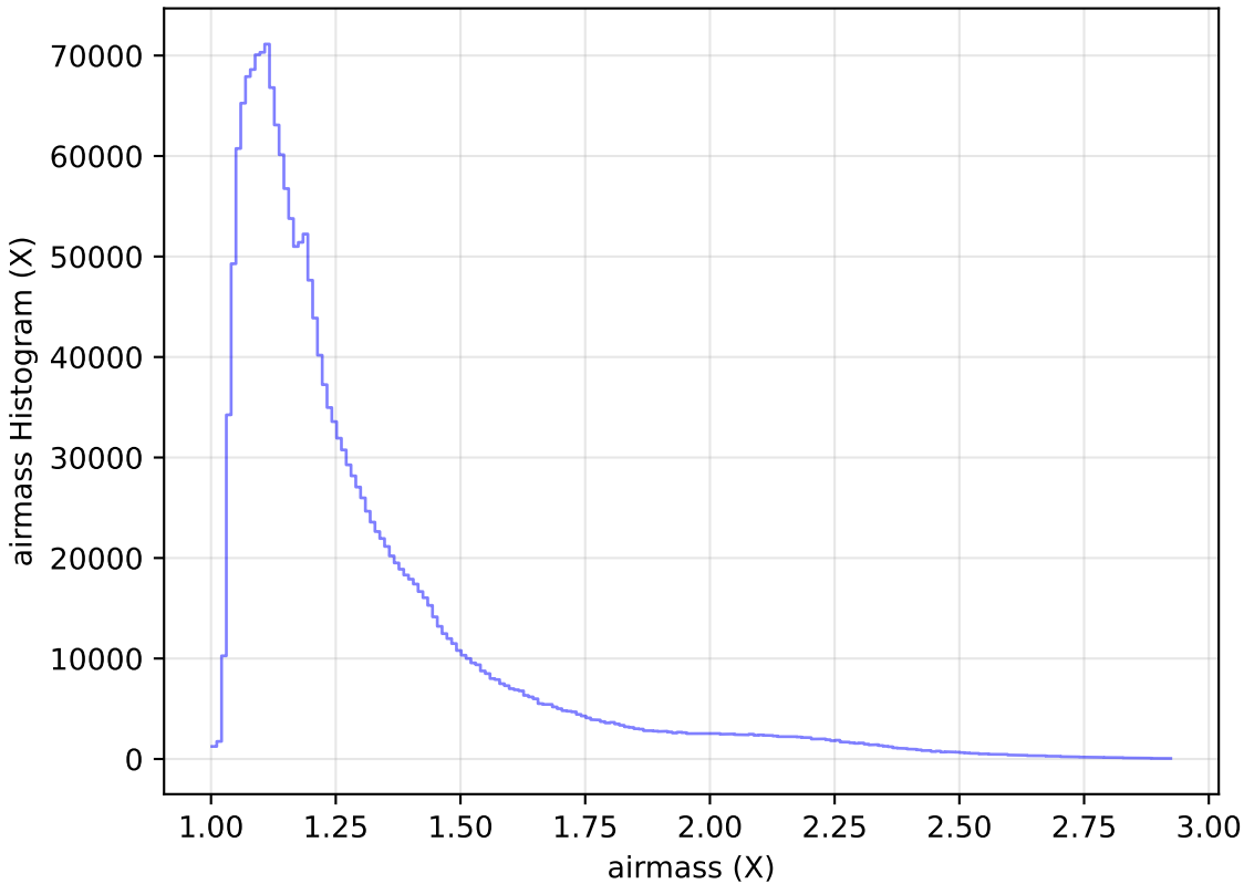
too_elab_r64_d2_gz_v3.4_10yrs WFD all bands: airmass Histogram
