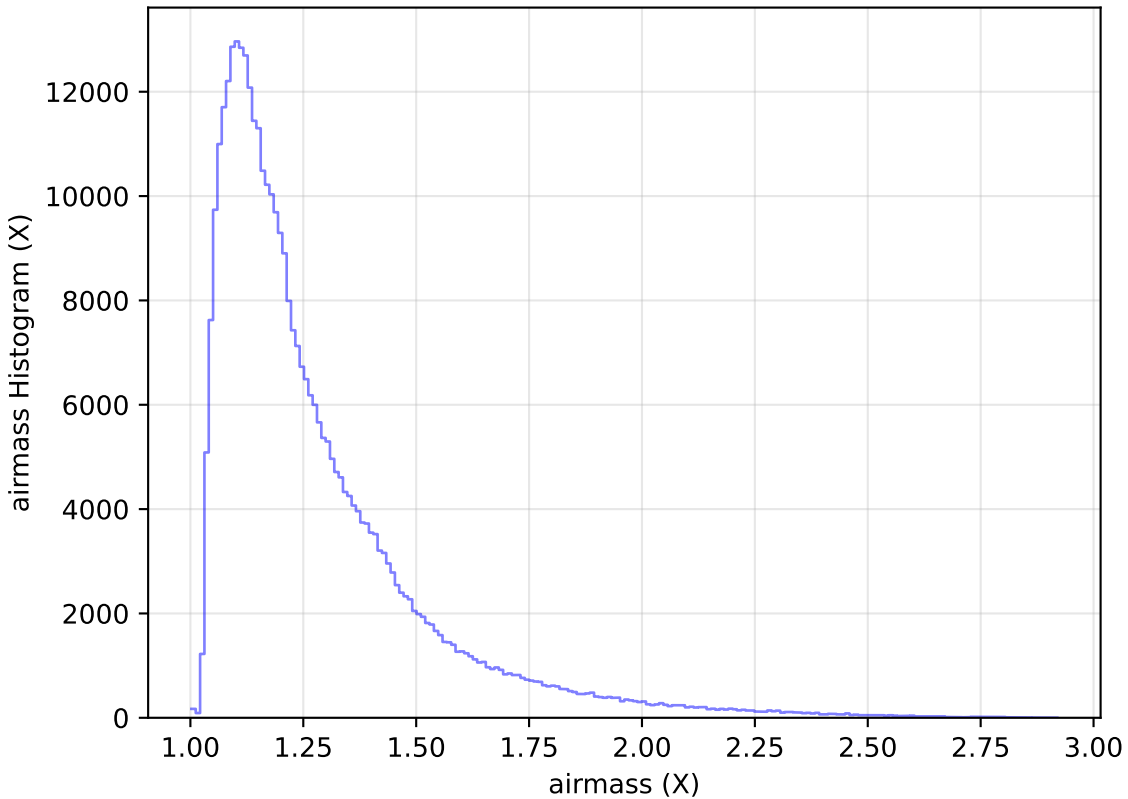
too_elab_r64_d2_gz_v3.4_10yrs All sky y band: airmass Histogram
